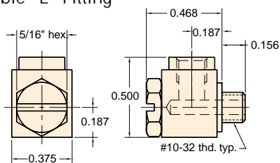
Adjustable "L" Fitting
